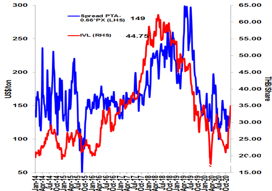
Spread PTA-0.66*PX vs IVL
