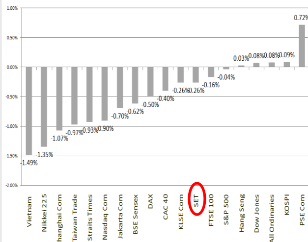
% above ema10-day : average -0.455%
