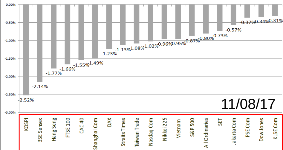
% above ema10-day : average -1.132%
